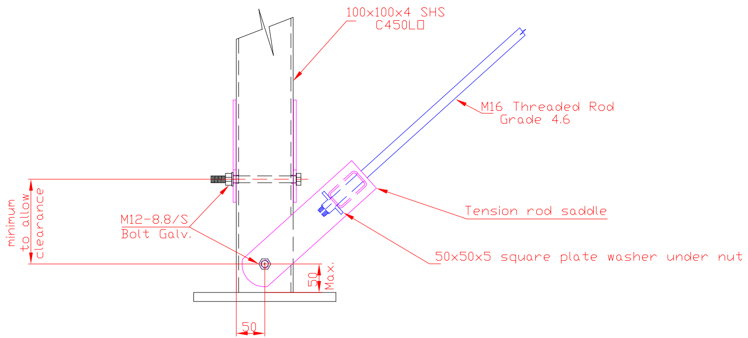
Bracing Bottom Detail (Outer Column)
