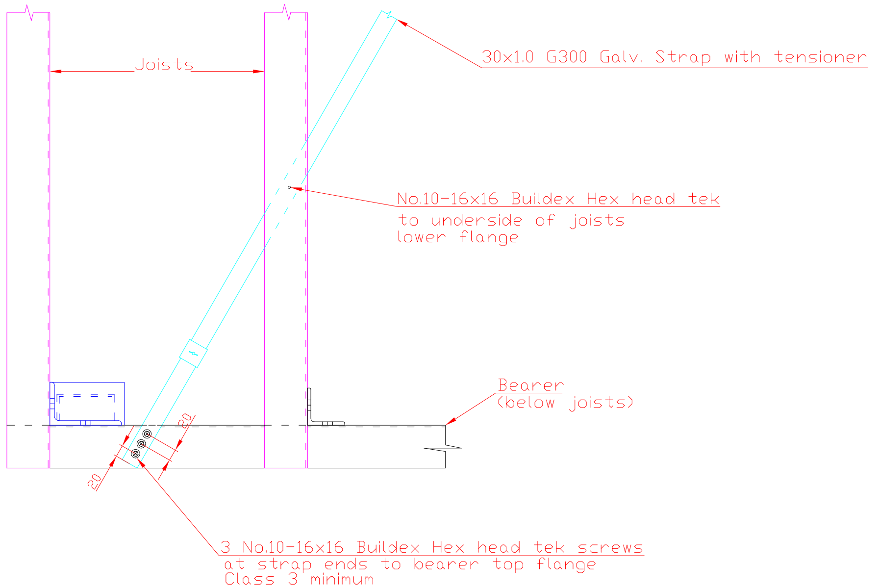
Floor Bracing Detail
